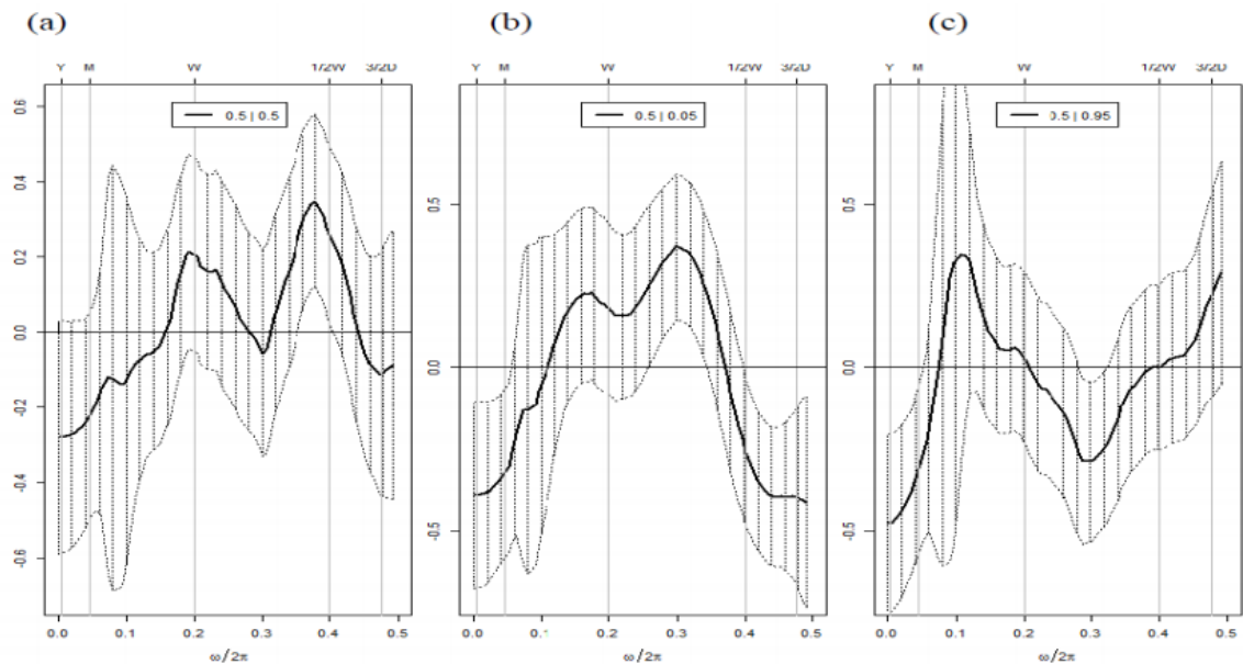
Figure 7: The quantile coherency estimates between the vaccination rate and sectoral stock return (consumer discretionary)
